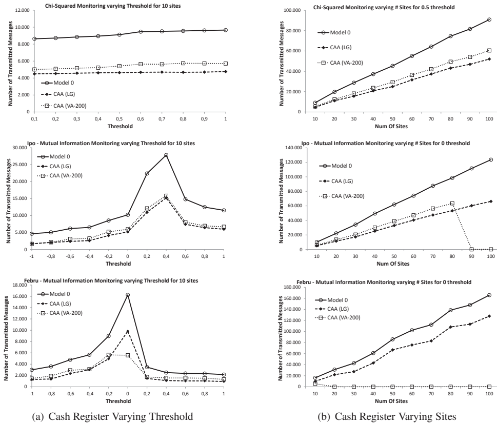
Fig. 8. Corpus Data Set: Performance of our Techniques in the Cash Register Streaming Paradigm
