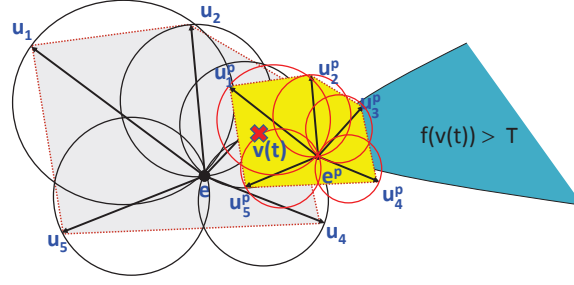
Fig. 3. The red balls demonstrate the local constraints of sites when using a sample good predictor. A good predictor results in the tighter convex hull Conv(u_1^p(t), \dots, u_n^p(t)) (depicted in yellow). Here, fewer synchronizations are not guaranteed, since \bigcup_{i=1}^n B_{\frac{e^p(t)-u_i^p(t)}{2}} crosses the threshold before \bigcup_{i=1}^n B_{\frac{e-u_i(t)}{2}} .
