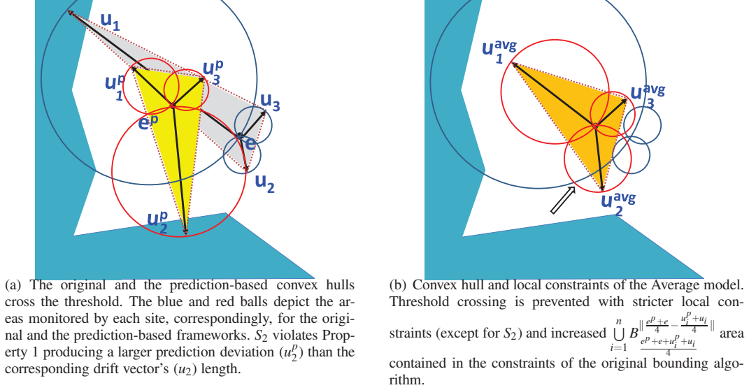
Fig. 4. The effect of the Average model adoption
