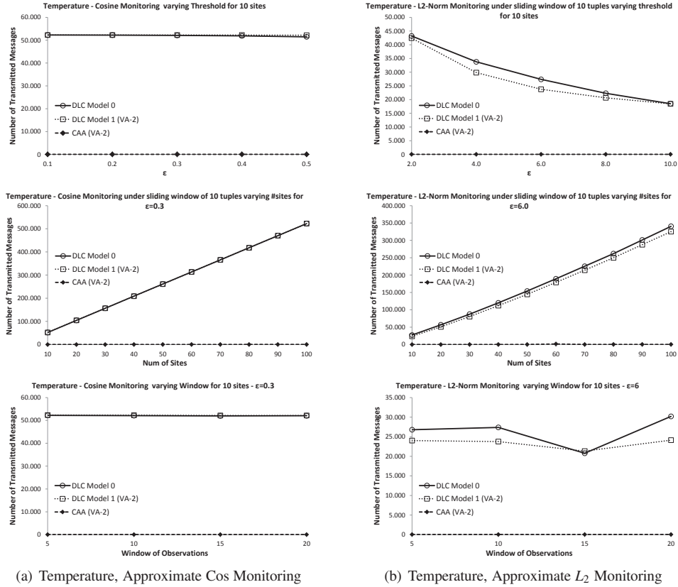
Fig. 12. Weather Data Set - Temperature: Approximate Query Answering Performance
